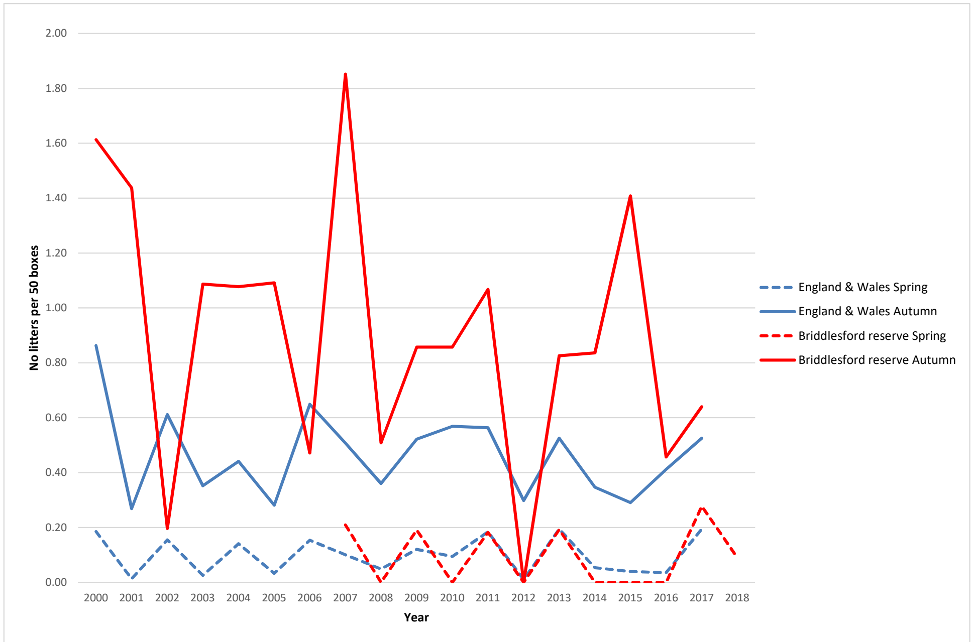
Total number of LITTERS of dormice in Spring and Autumn recorded in UK regions compared to Briddlesford Reserve per 50 boxes
